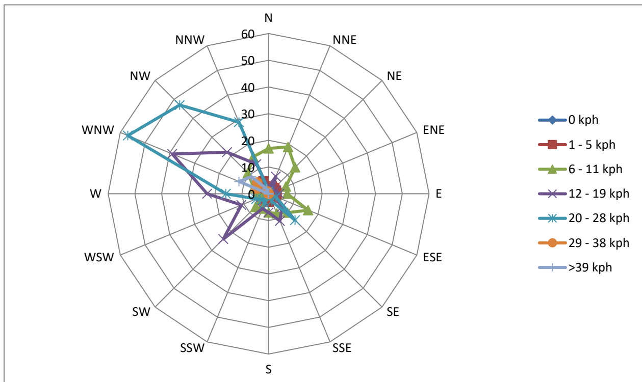
Figure 6-16: April Windrose (1 hour Average, 30m)
