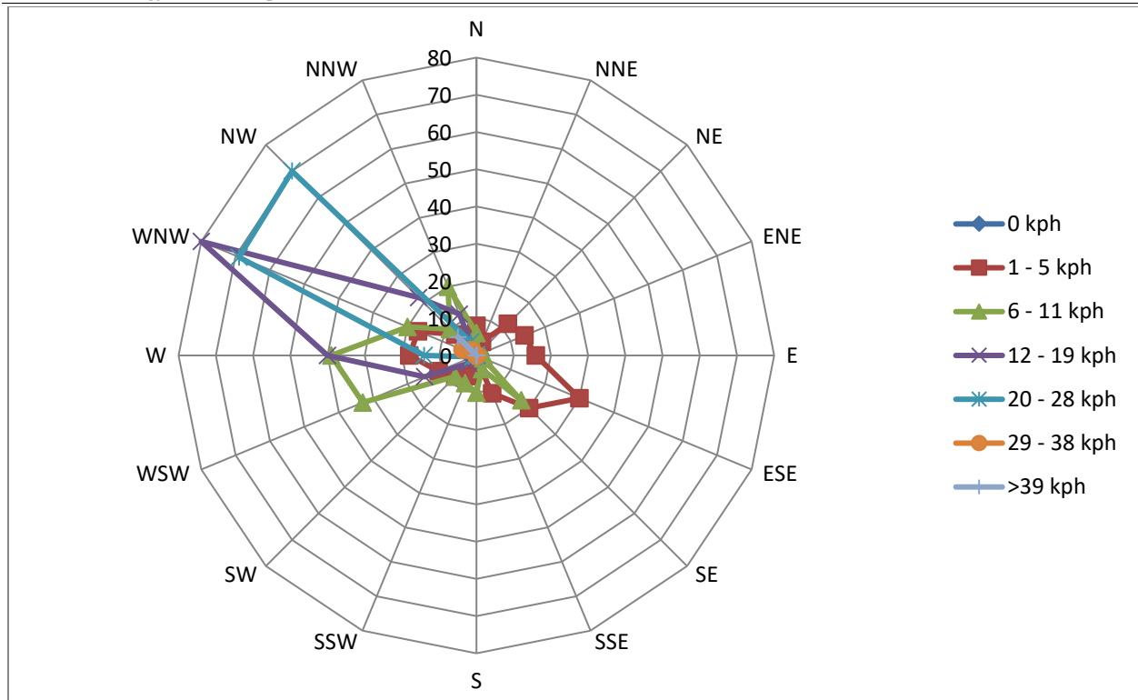
Figure 6-19: July Windrose (1 hour Average, 30m)
