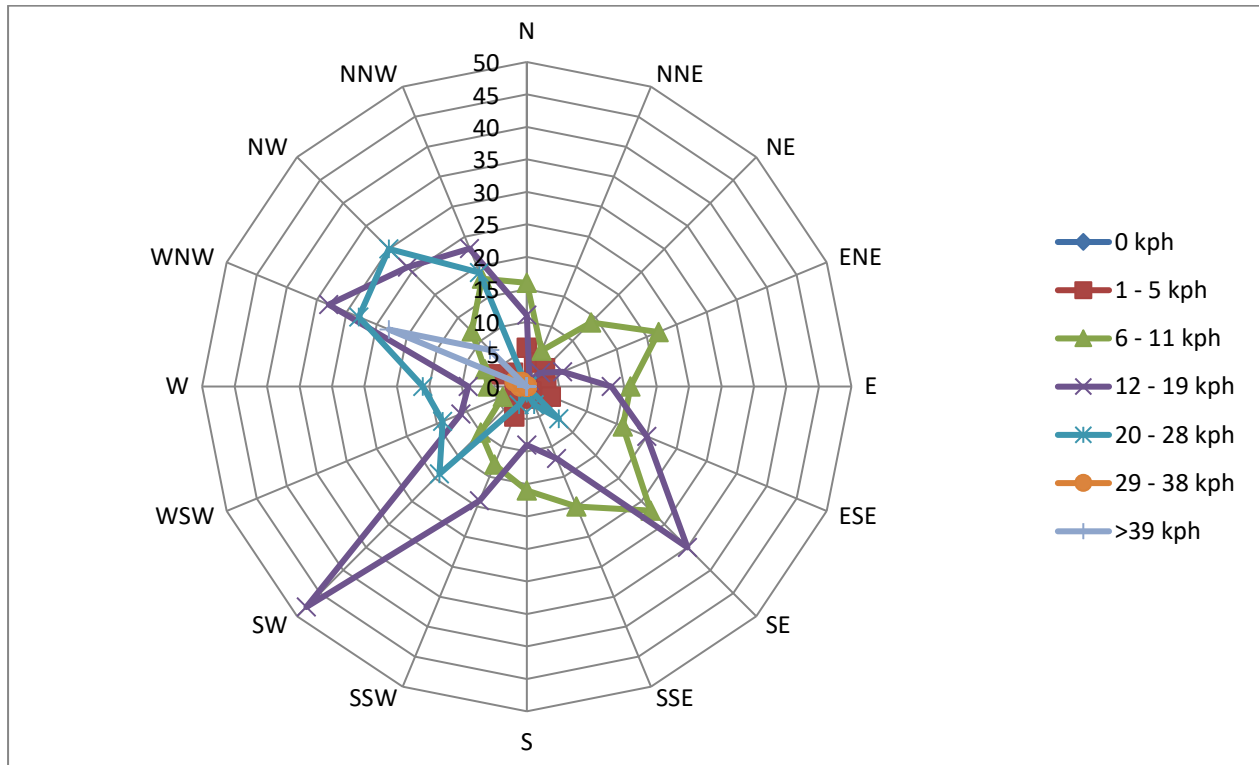
Figure 6-15: March Windrose (1 hour Average, 30m)
