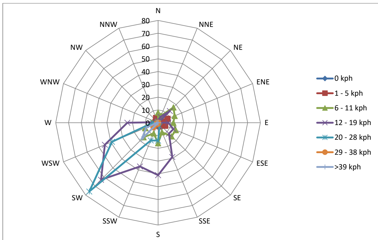
Figure 6-22: October Windrose (1 hour Average, 30m)
