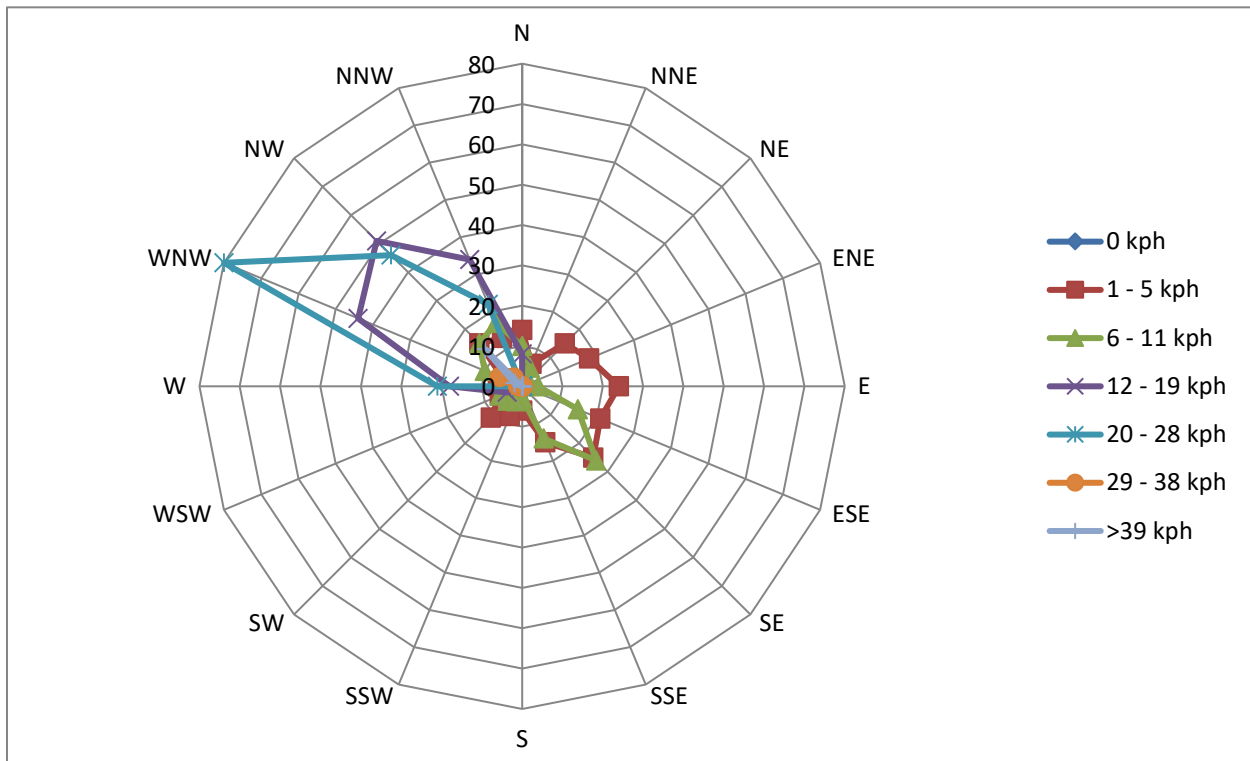
Figure 6-5: May Windrose (1 hour Average)
