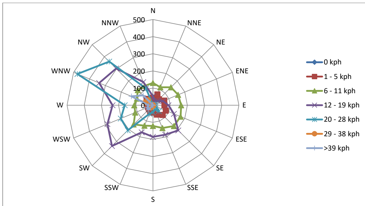
Figure 6-26: Annual Windrose (1 hour Average, 30m)
