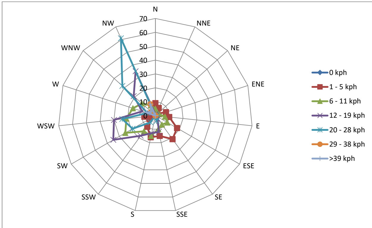
Figure 6-13: January Windrose (1 hour Average, 30m)
