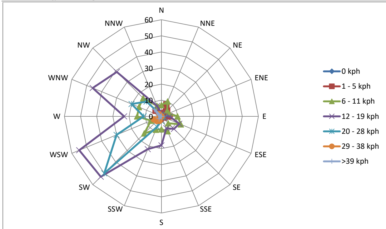
Figure 6-21: September Windrose (1 hour Average, 30m)
