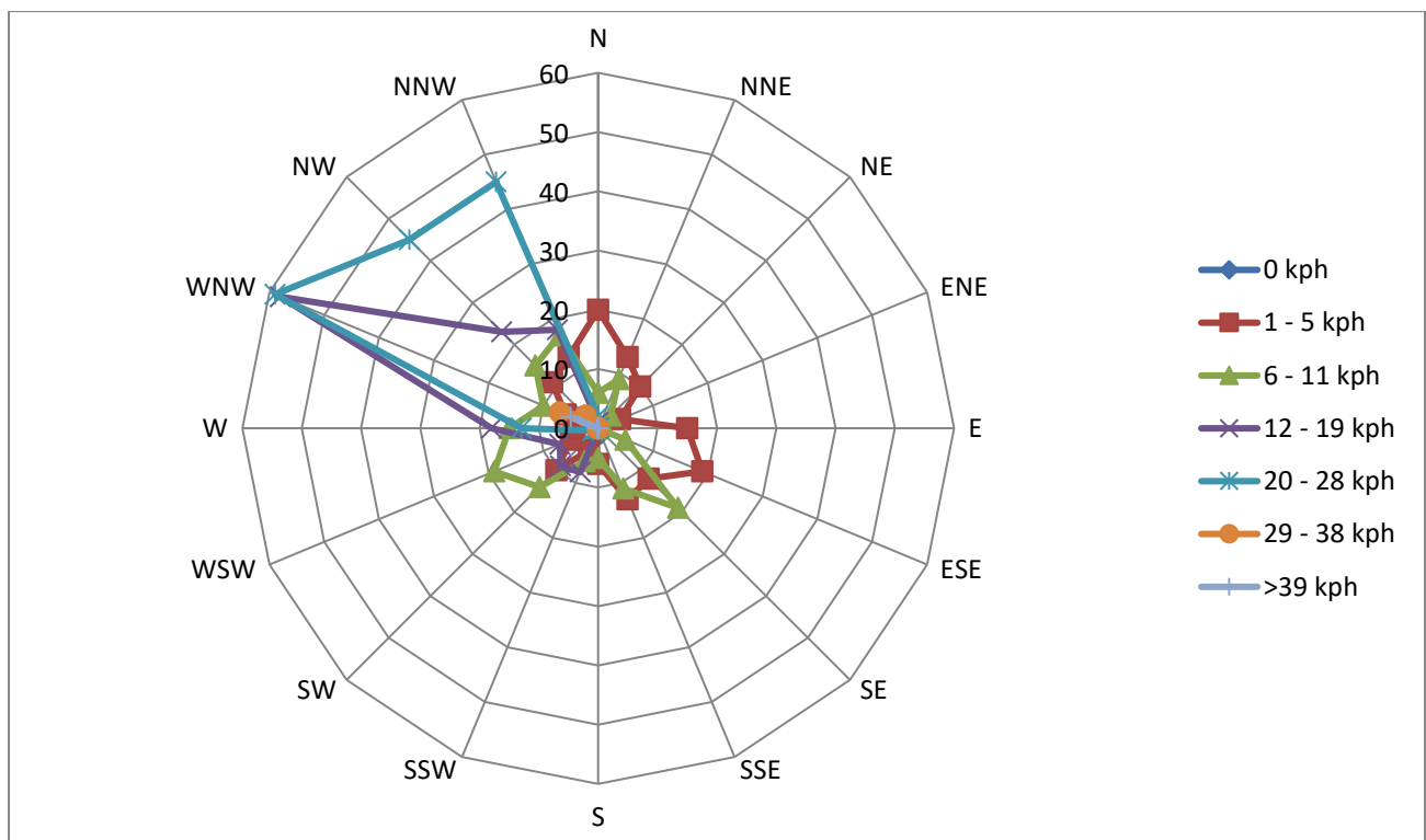
Figure 6-4: April Windrose (1 hour Average, 10 m)
