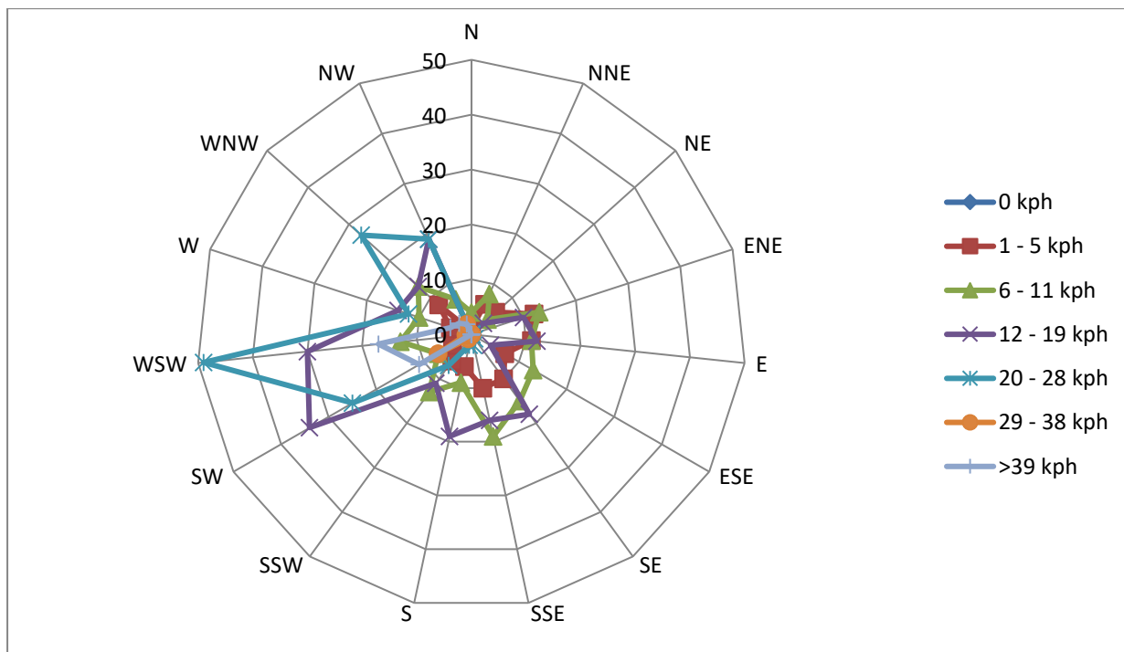
Figure 6-24: December Windrose (1 hour Average, 30m)
