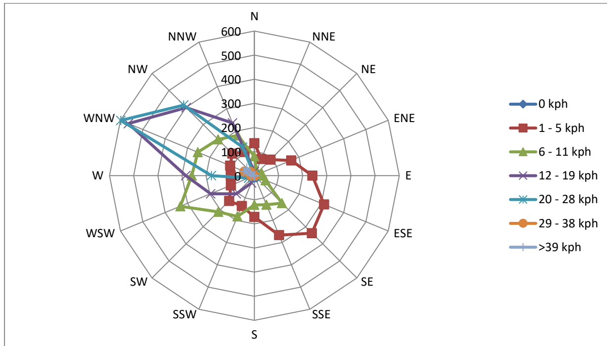
Figure 6-25: Annual Windrose (1 hour Average, 10m)
