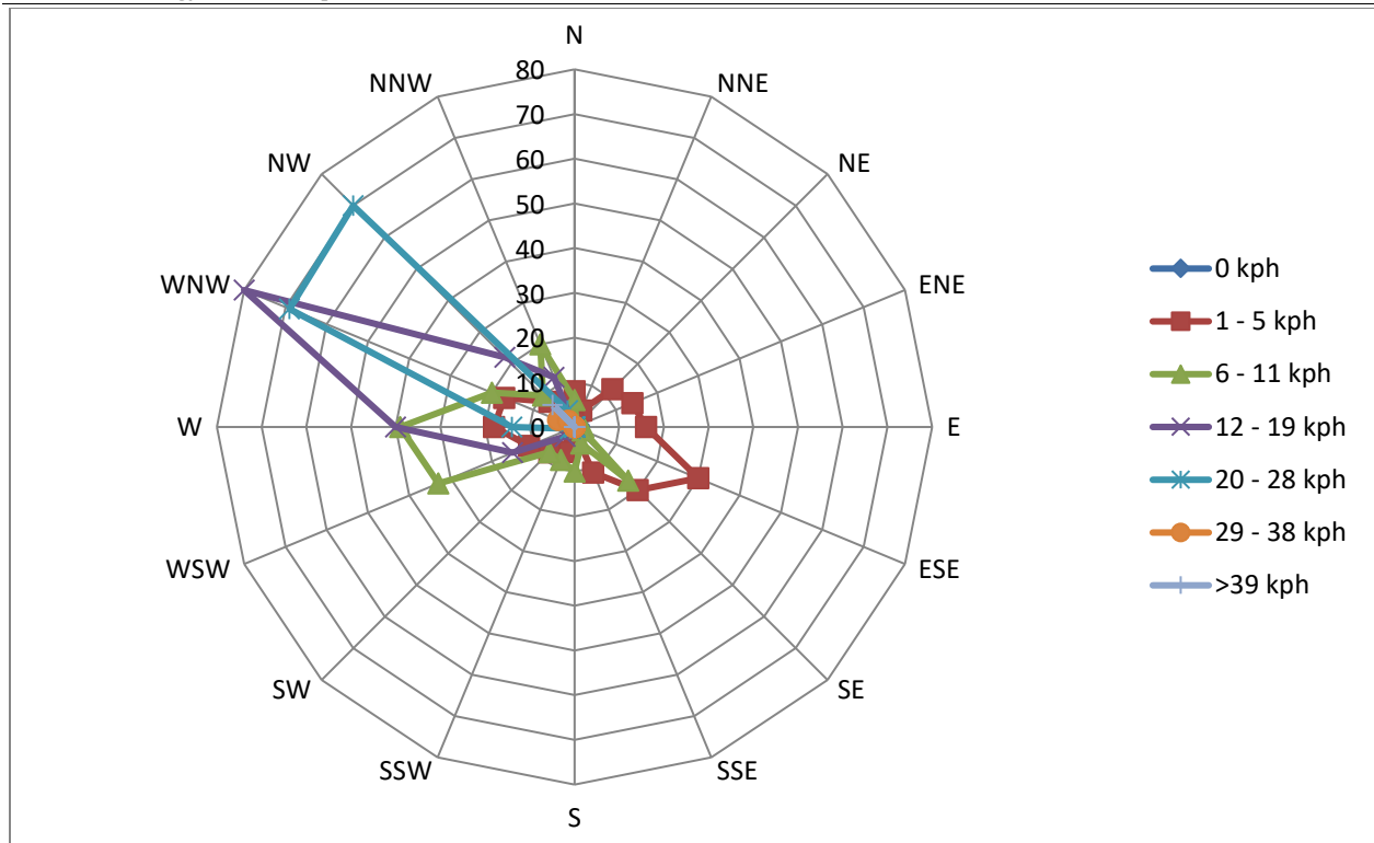
Figure 6-7: July Windrose (1 hour Average, 10m)
