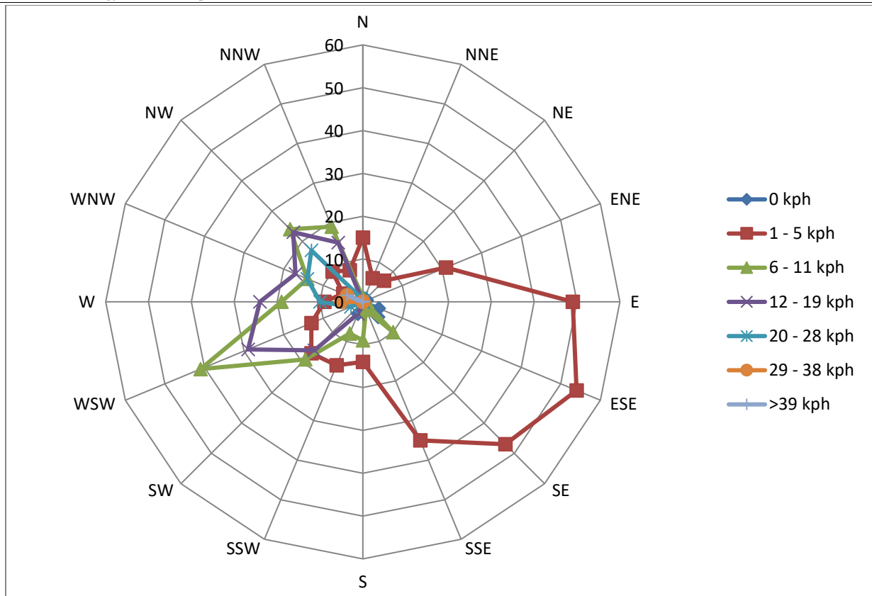
Figure 6-11: November Windrose (1 hour Average, 10m)
