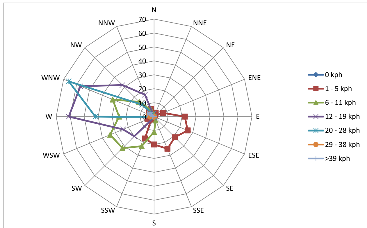
Figure 6-10: October Windrose (1 hour Average, 10m)
